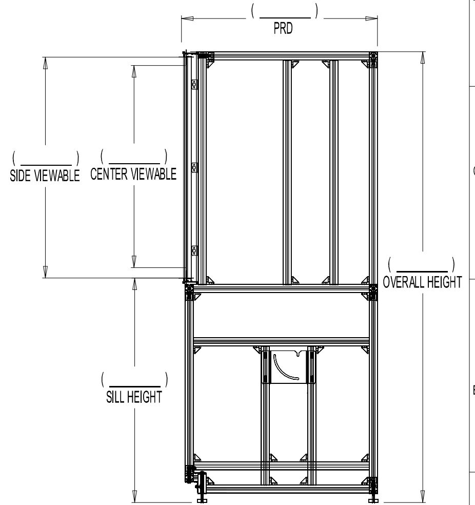
SECTION (SIDE VIEW)
