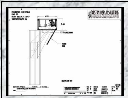
DESIGN – SECTION VIEW
